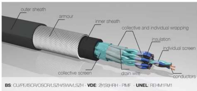
Instrumentation Cables
