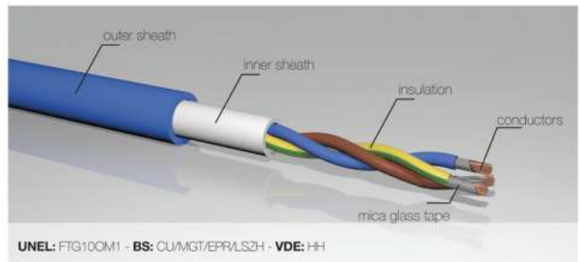
Fire Resistant
