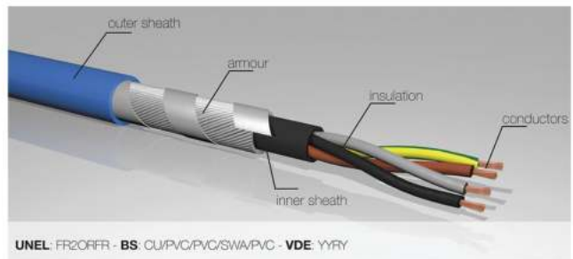
Power Cable
